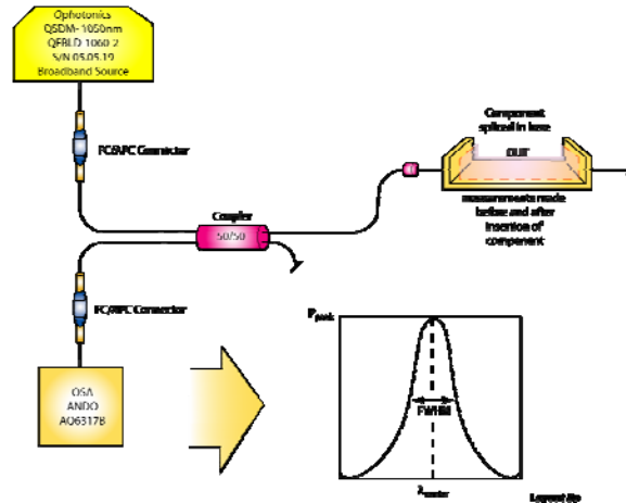
Figure 3. FBG LI performance measurement setup.
