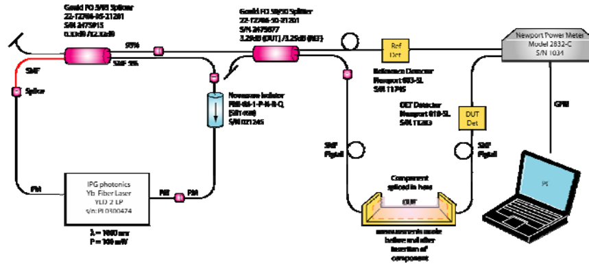
Figure 2. IL (and isolation) performance measurement setup.
