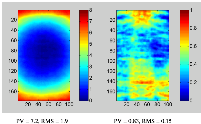
Fig. 8. Initial distorted wavefront with DM (left) and closed-loop corrected wavefront (right) after four passes through the system.
