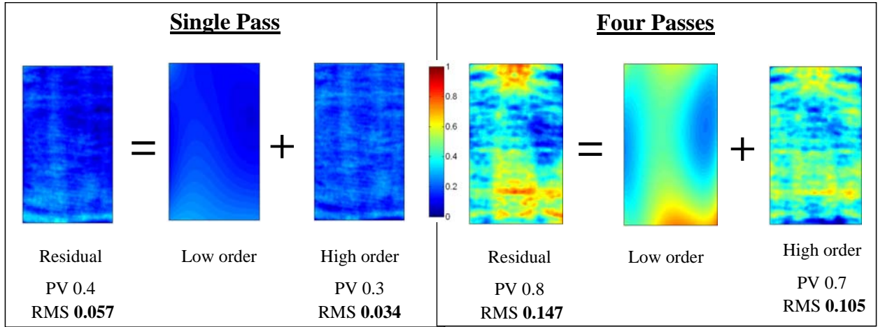
Fig. 9: Legendre decomposition results for single pass (left) and four pass corrected wavefront.
