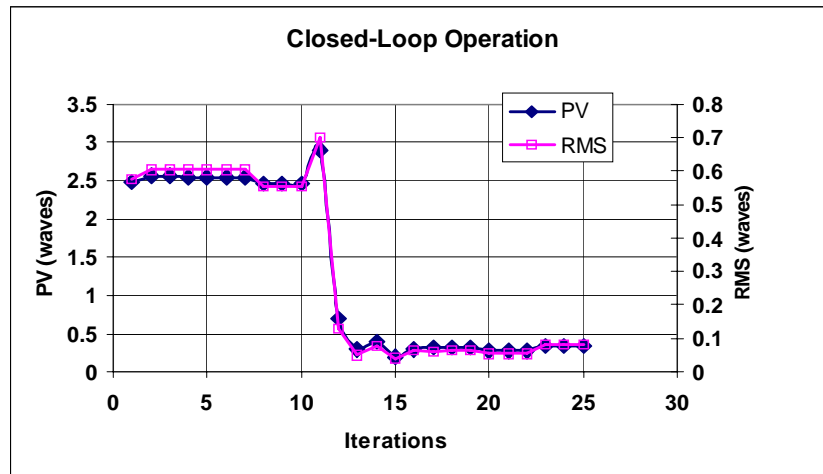
Fig. 4. Closed loop operation of the DM system for a 45 x 75 mm beam, improving RMS from 0.6 waves to 0.04 waves.
