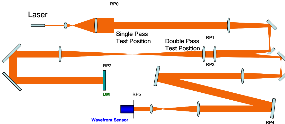
Fig. 2. Mercury offline diagnostic beam layout
