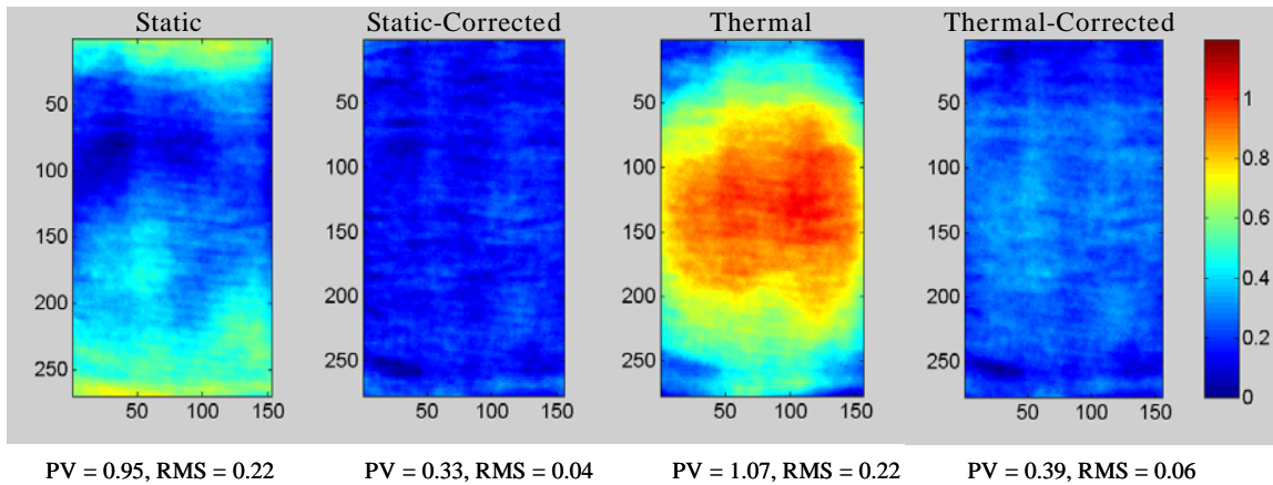
Fig. 7: Static wavefront without DM, closed-loop corrected static wavefront, 15 minutes thermal wavefront, and closed-loop corrected thermal wavefront after single pass through the amplifier system.
