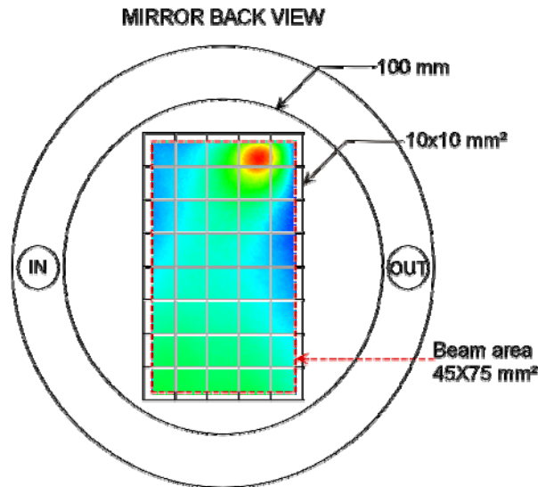
Fig. 1. Mercury Laser's 100 mm diameter DM with 40+1 actuators arranged in 5x8 configuration. A typical influence function is overlay over the actuators.
