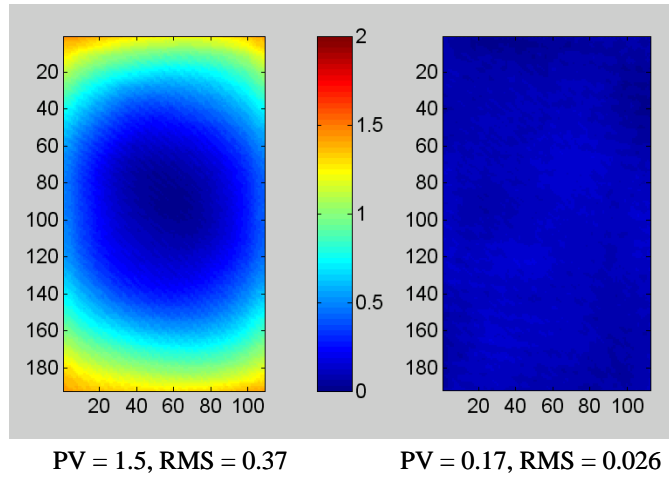
Fig. 3. Initial wavefront (RMS = 0.37) and final wavefront (RMS = 0.026) after successful closed-loop.
