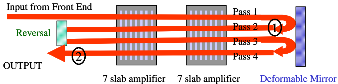
Fig. 6: Mercury DM online experiment layout. The sensor is placed at position 1 for single pass DM correction and position 2 for four-pass DM correction. Beam is flipped horizontally after the reversal.
