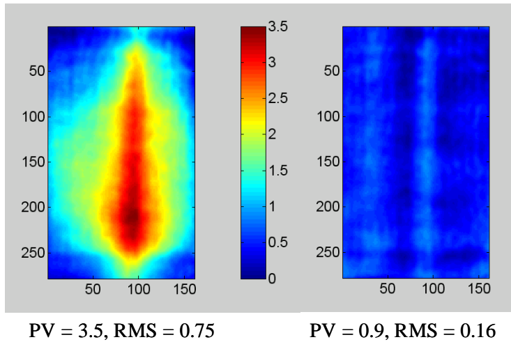
Fig. 5. Wavefront of uncorrected beam double passing through phase plate with bond line before (left) and after correction (right) by the DM
