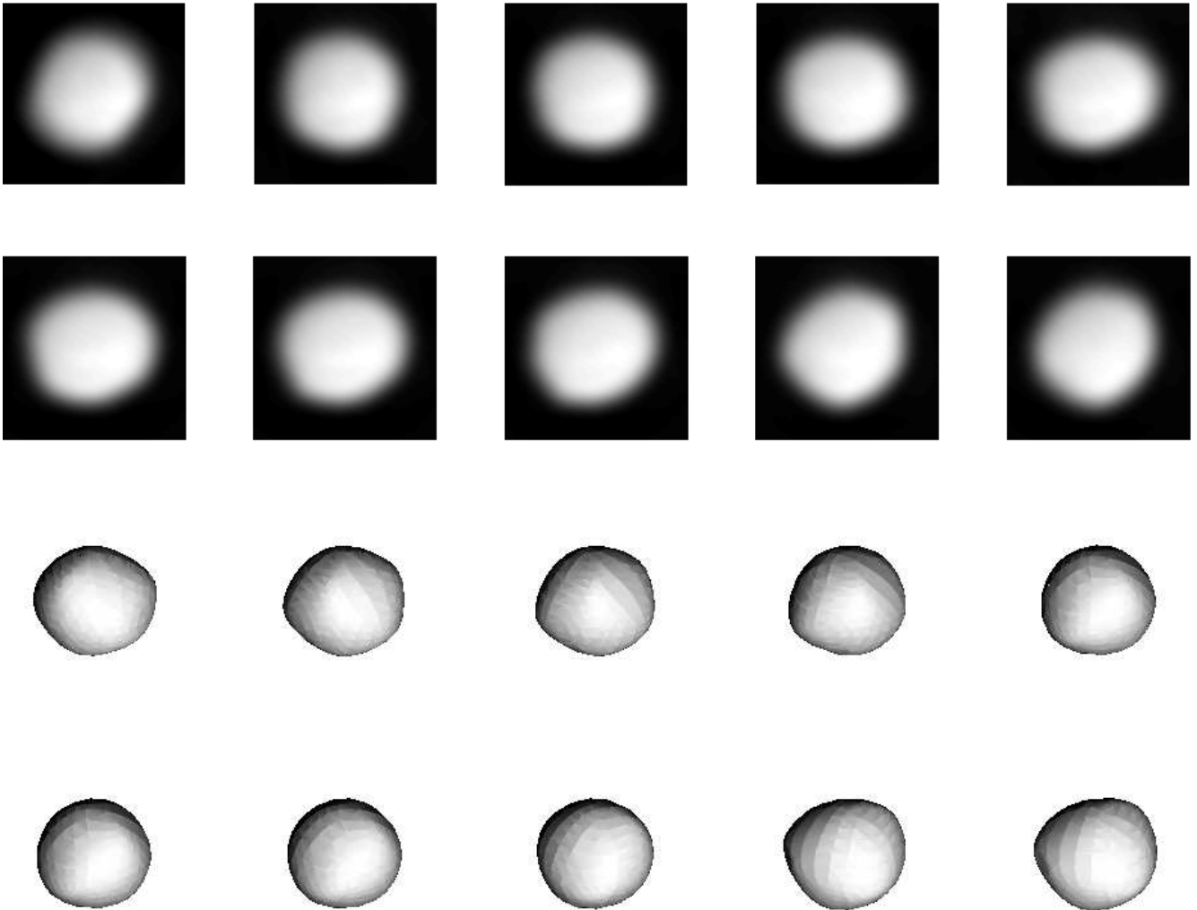
Figure 3. Deconvolved images of 2 Pallas and models from lightcurve inversions.
