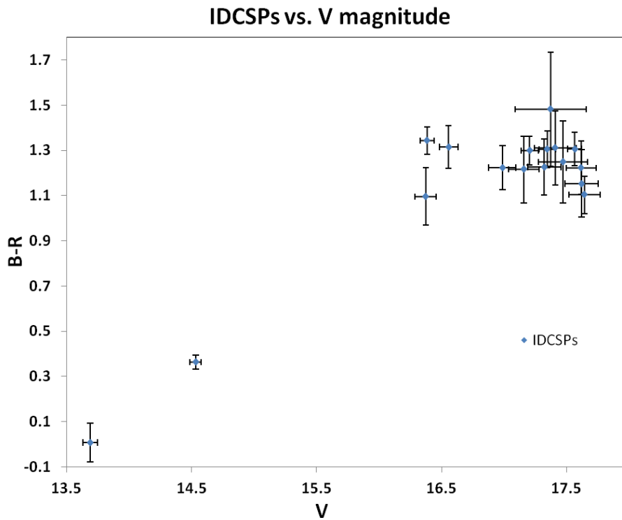
Fig. 3 B-R color versus V magnitude.
