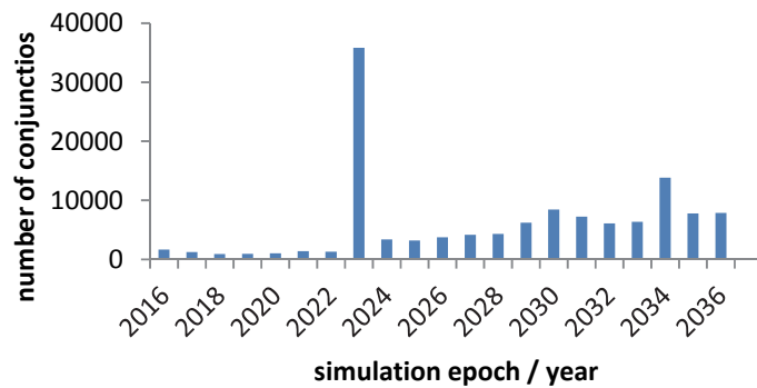
Figure 8: Number of conjunctions with a probability of collisions larger than 10^{-4} for one run of the optimistic “New Space” scenario.
