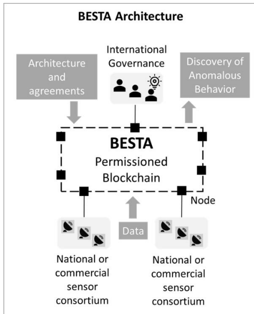
Fig 3. BESTA Architecture
