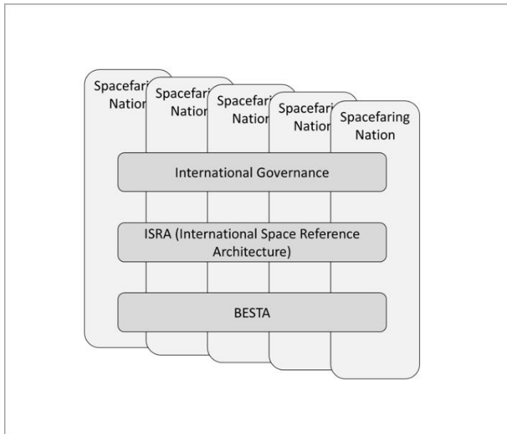
Fig. 5 BESTA Governance
