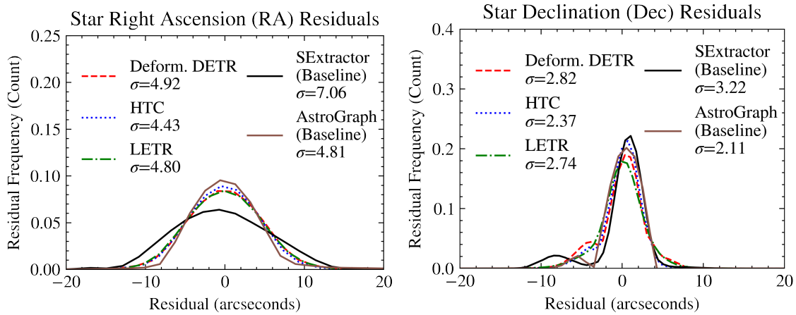
Fig. 6: Star centroid residual distributions in world space. Standard deviations are included in the legend.
