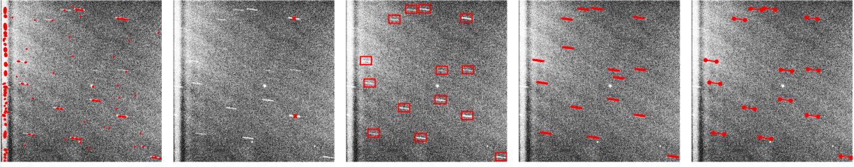
Fig. 3: A random StarNet image with star detections. From left to right: SExtractor isophotal ellipses, AstroGraph centroids, Deformable DETR bounding boxes, HTC instance segmentations, and LETR line segmentations.
