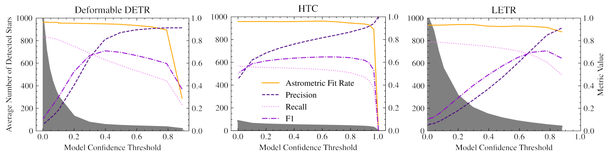
Fig. 4: Comparing astrometric fit rate to model performance metrics for (a) Deformable DETR (b) HTC (c) LETR. The average number of detected stars at a given confidence threshold is shown in gray.
