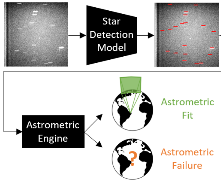
Fig. 1: The astrometric image processing pipeline. A star detection model accepts an astronomical image as input and produces detected star positions. The detected star positions are passed to an astrometric engine, which uses the ratios between the star positions to match detected stars to real world catalog stars. The output of this pipeline is either an astrometric fit (if the detected stars could be matched to the celestial sphere) or an astrometric failure (if the detected stars could not).
